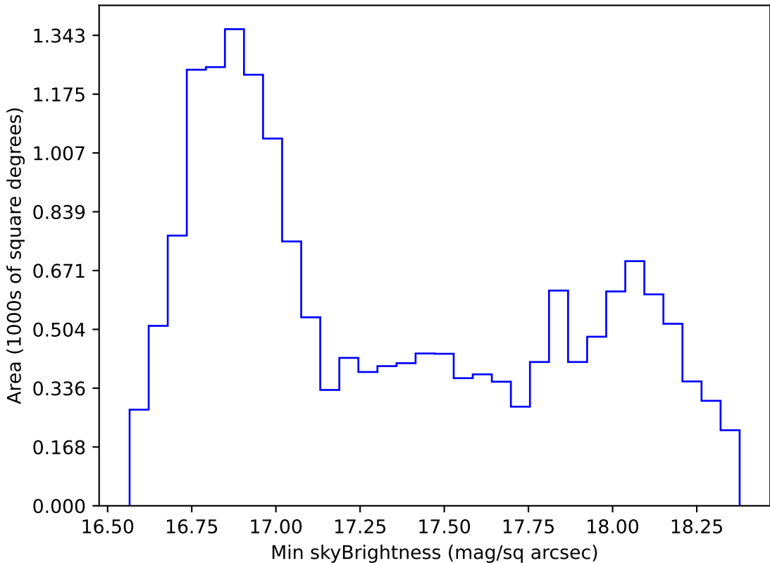
roll_pause_mjdp60_v3.4_10yrs WFD z band: Min skyBrightness
