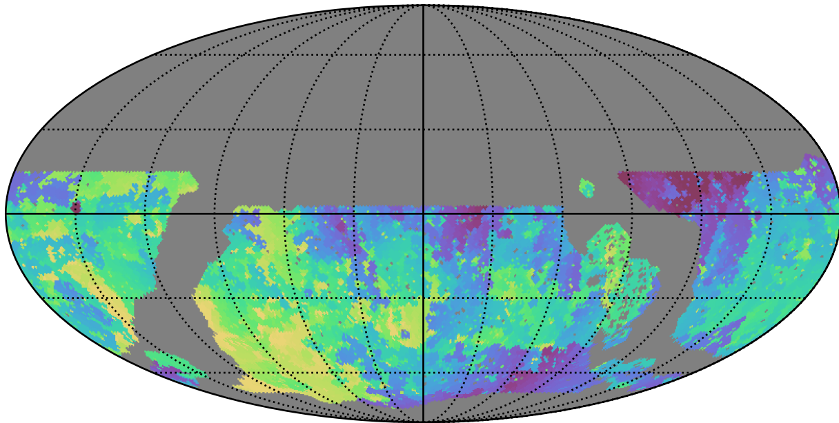
roll_pause_mjdp60_v3.4_10yrs WFD u band: Min skyBrightness
