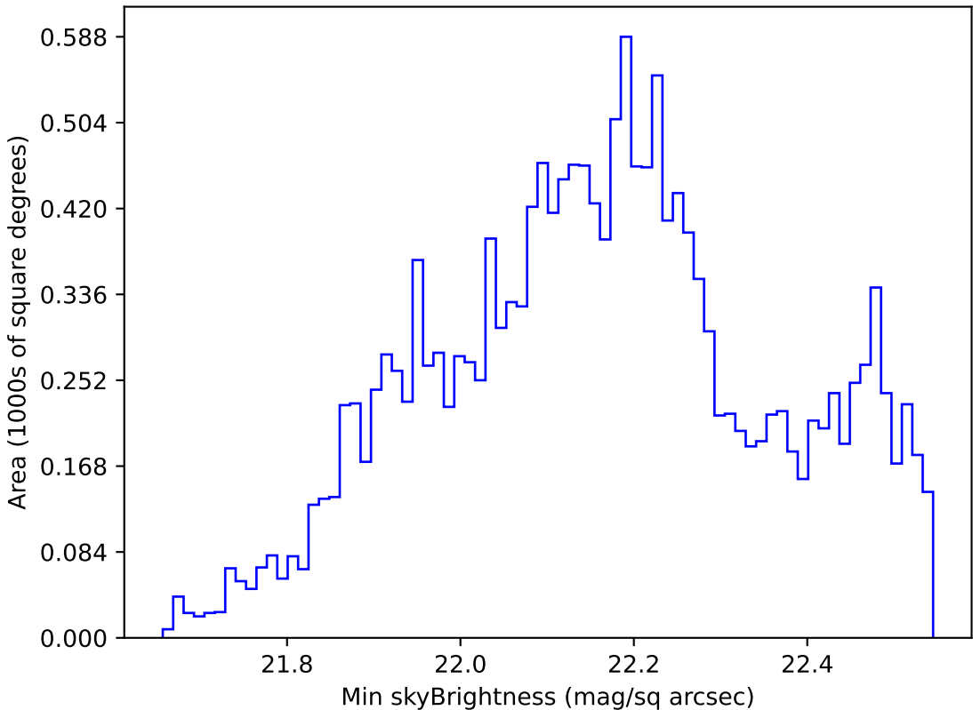
roll_pause_mjdp60_v3.4_10yrs WFD u band: Min skyBrightness
