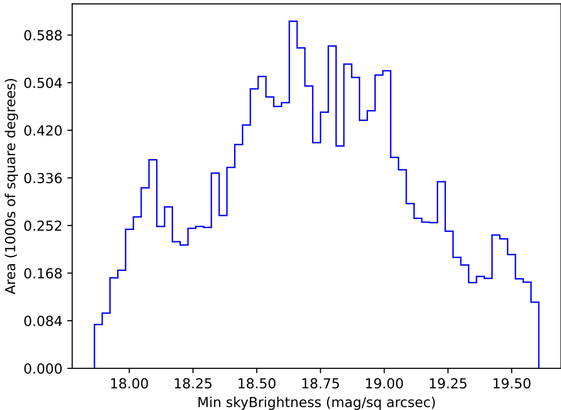
roll_pause_mjdp60_v3.4_10yrs WFD r band: Min skyBrightness
