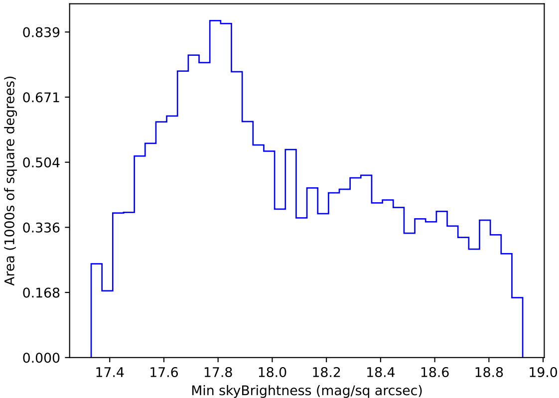
roll_pause_mjdp60_v3.4_10yrs WFD i band: Min skyBrightness
