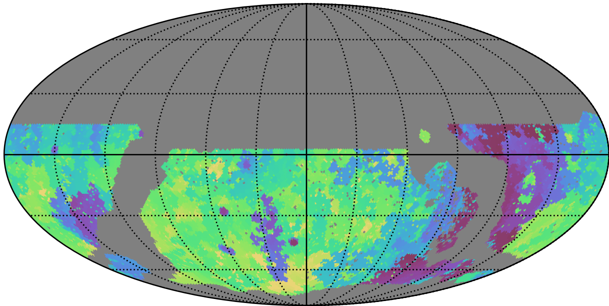
roll_pause_mjdp60_v3.4_10yrs WFD g band: Min skyBrightness
