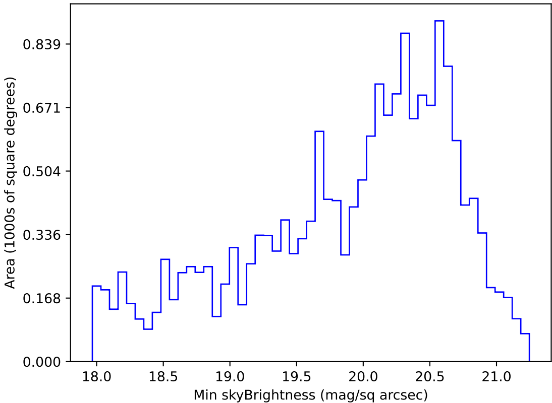
roll_pause_mjdp60_v3.4_10yrs WFD g band: Min skyBrightness
