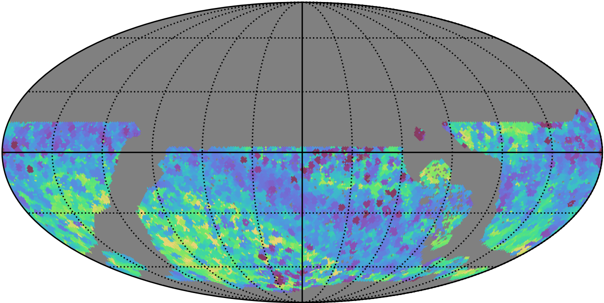
roll_pause_mjdp60_v3.4_10yrs WFD all bands: Min skyBrightness
