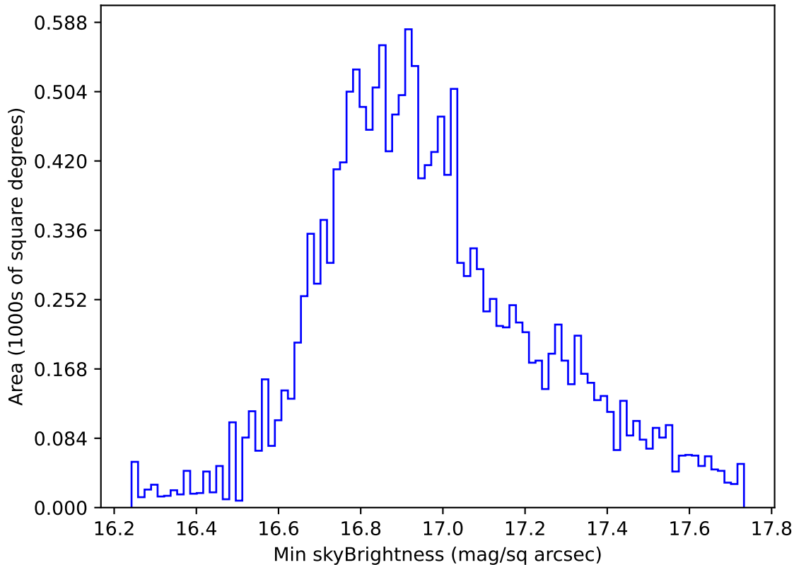
roll_pause_mjdp60_v3.4_10yrs WFD all bands: Min skyBrightness
