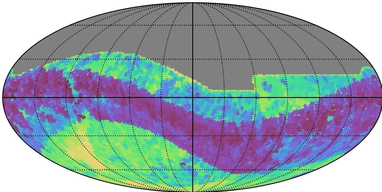
roll_pause_mjdp60_v3.4_10yrs All sky z band: Min skyBrightness
