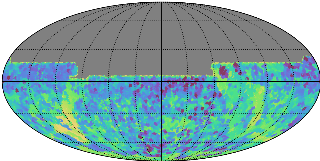
roll_pause_mjdp60_v3.4_10yrs All sky y band: Min skyBrightness
