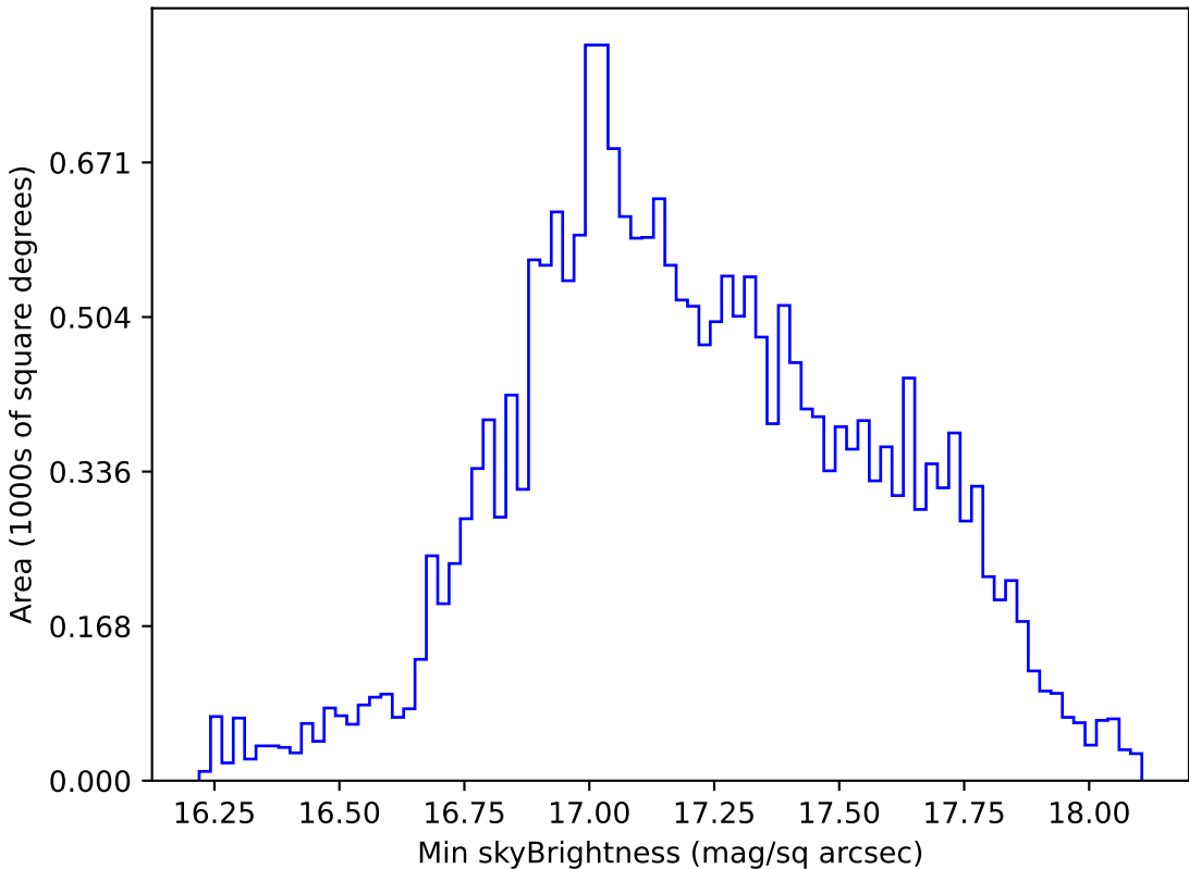
roll_pause_mjdp60_v3.4_10yrs All sky y band: Min skyBrightness
