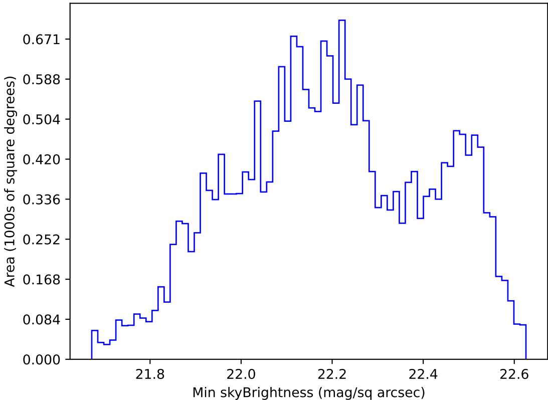
roll_pause_mjdp60_v3.4_10yrs All sky u band: Min skyBrightness
