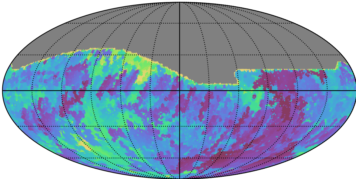
roll_pause_mjdp60_v3.4_10yrs All sky r band: Min skyBrightness
