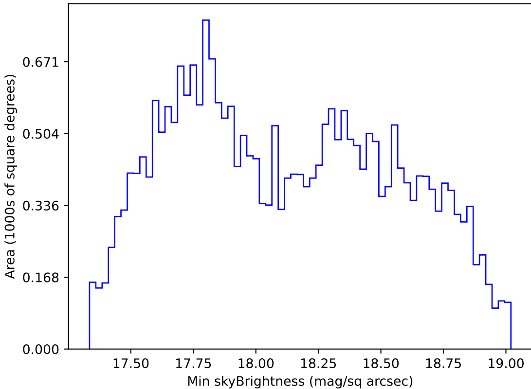
roll_pause_mjdp60_v3.4_10yrs All sky i band: Min skyBrightness
