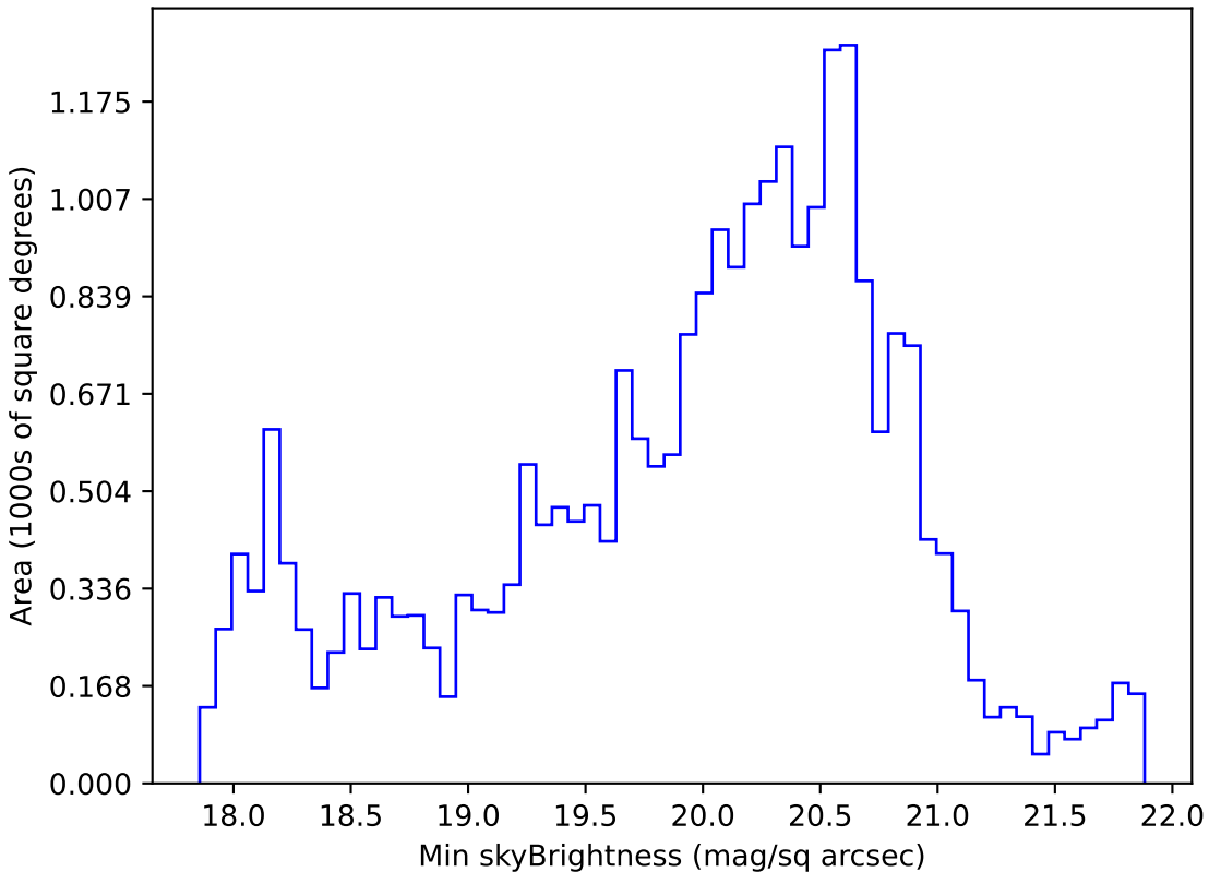
roll_pause_mjdp60_v3.4_10yrs All sky g band: Min skyBrightness
