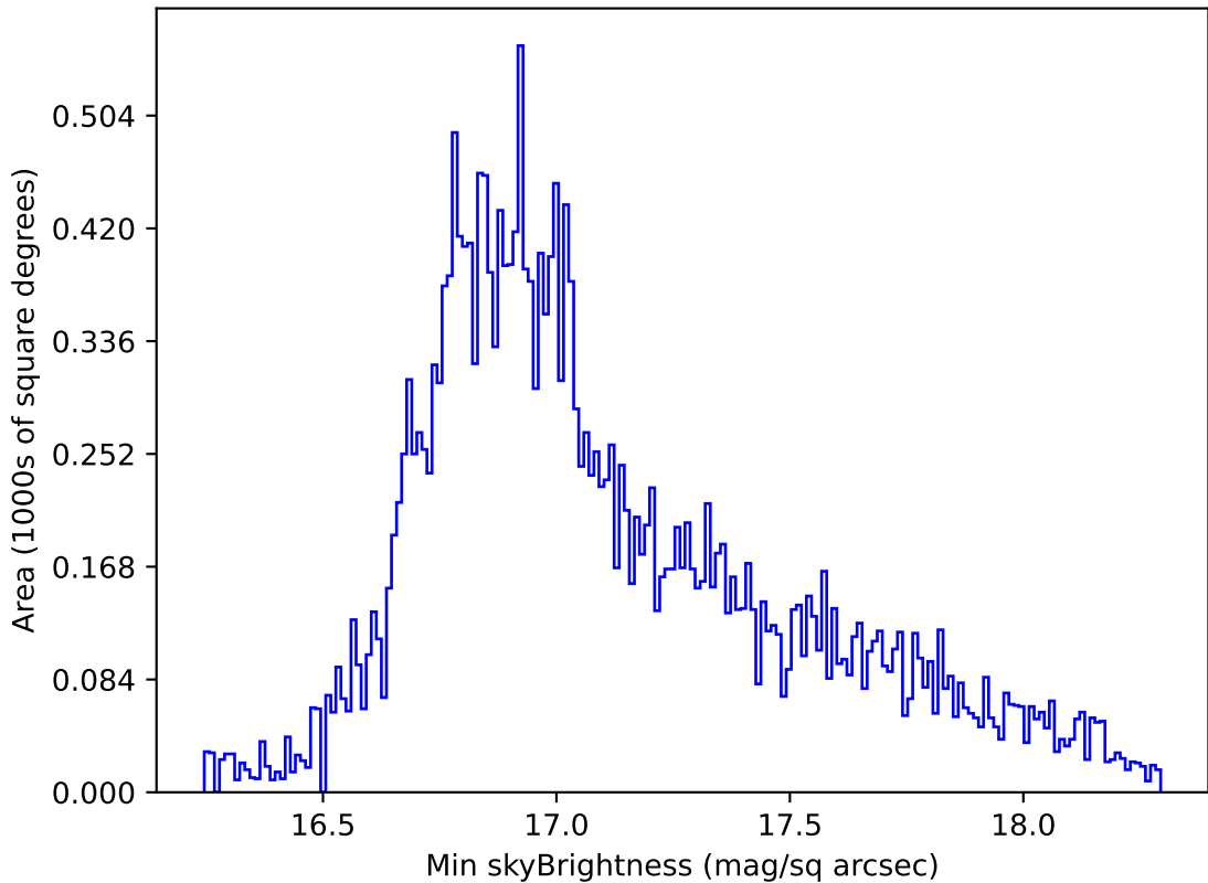
roll_pause_mjdp60_v3.4_10yrs All sky all bands: Min skyBrightness
