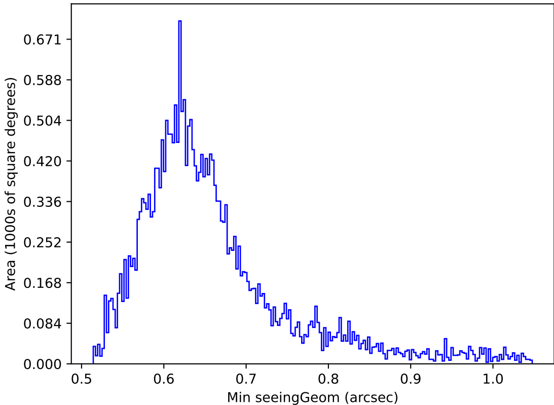
roll_pause_mjdp60_v3.4_10yrs Yr 1 z band: Min seeingGeom
