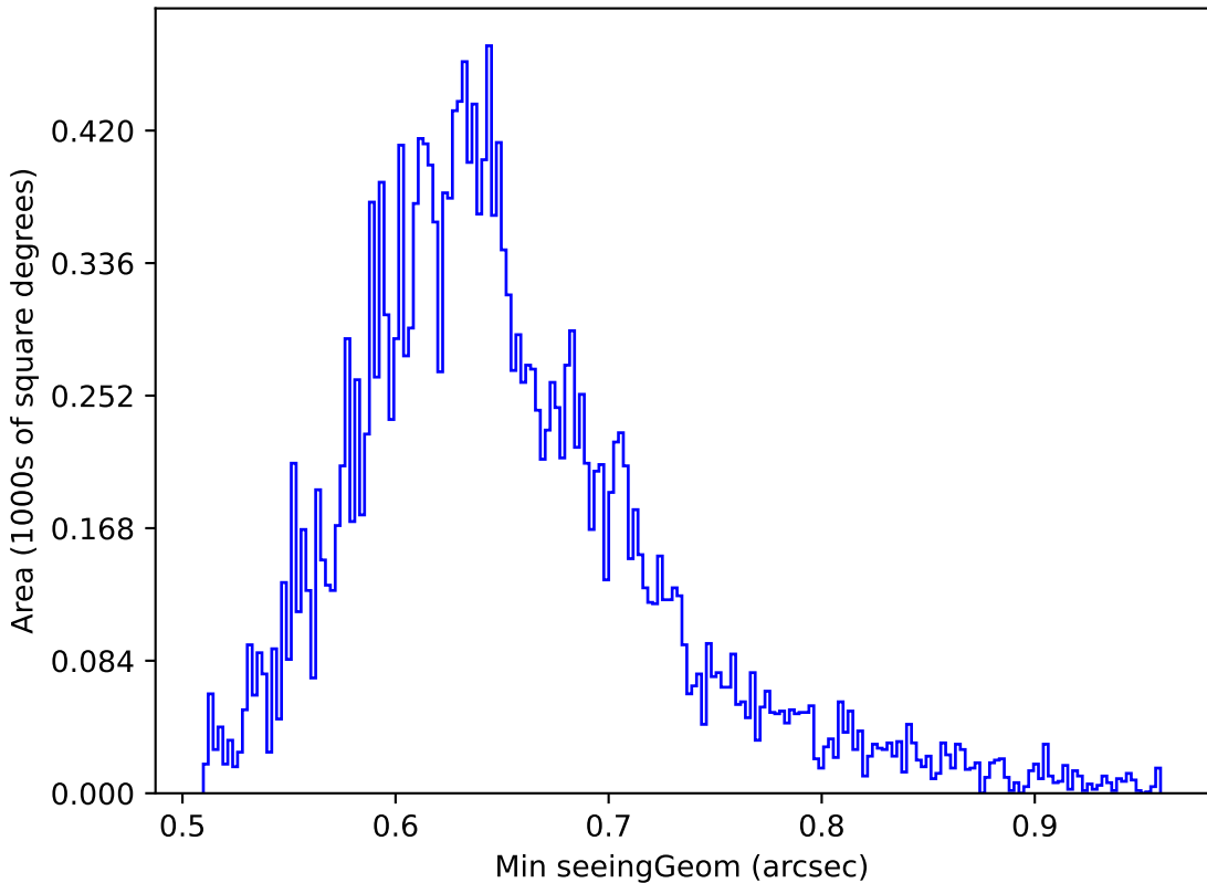
roll_pause_mjdp60_v3.4_10yrs Yr 1 y band: Min seeingGeom
