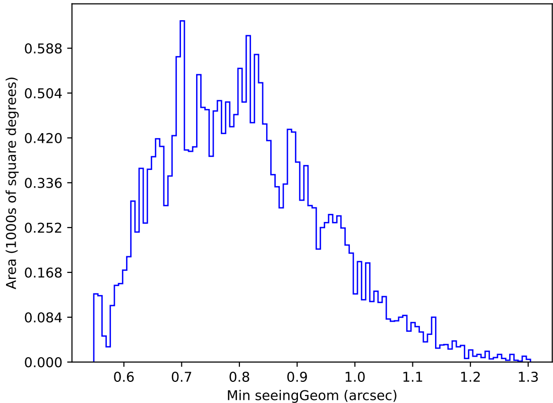
roll_pause_mjdp60_v3.4_10yrs Yr 1 u band: Min seeingGeom
