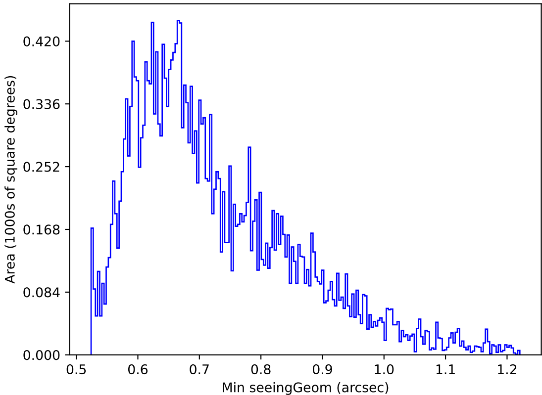
roll_pause_mjdp60_v3.4_10yrs Yr 1 g band: Min seeingGeom
