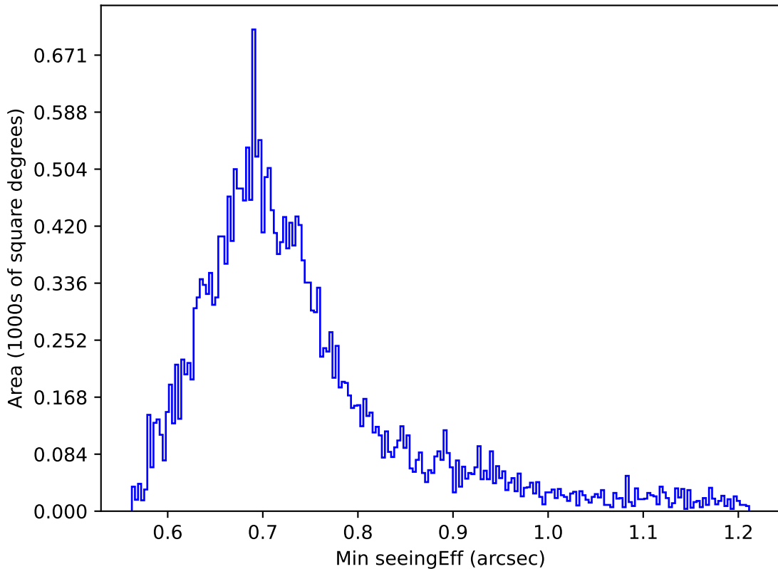
roll_pause_mjdp60_v3.4_10yrs Yr 1 z band: Min seeingEff
