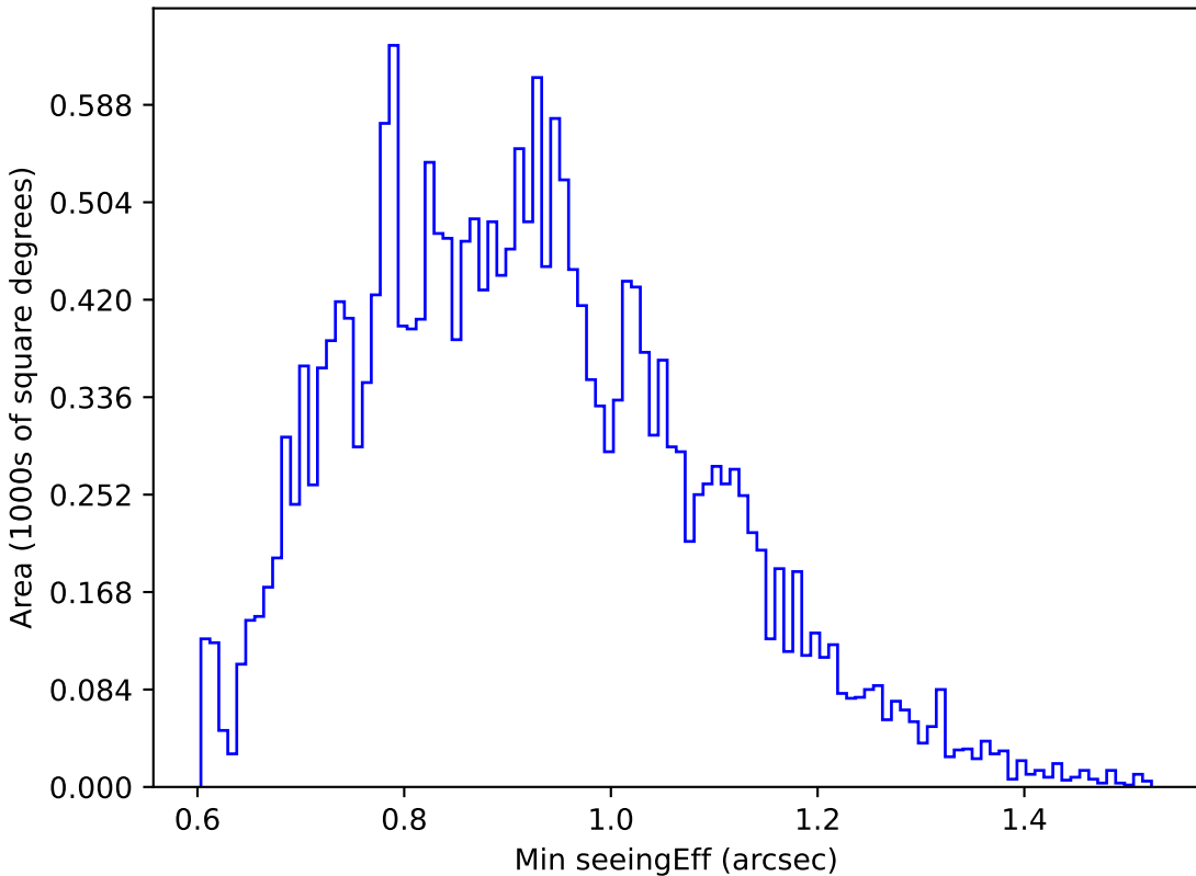
roll_pause_mjdp60_v3.4_10yrs Yr 1 u band: Min seeingEff
