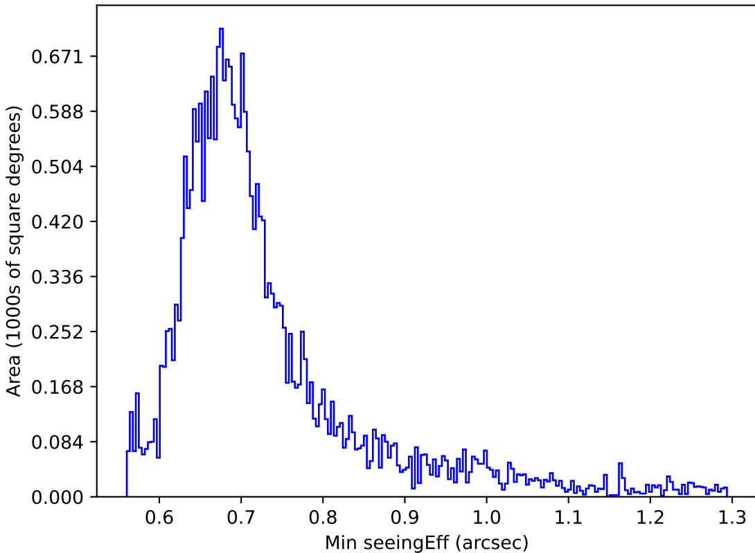
roll_pause_mjdp60_v3.4_10yrs Yr 1 r band: Min seeingEff
