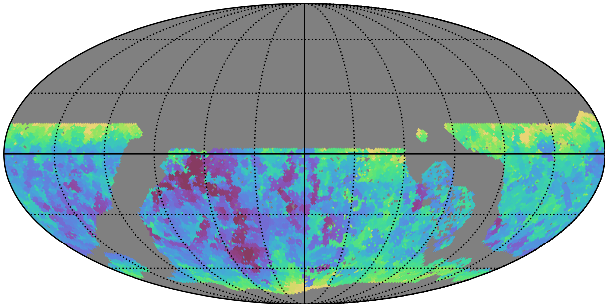
roll_pause_mjdp60_v3.4_10yrs WFD z band: Min seeingEff
