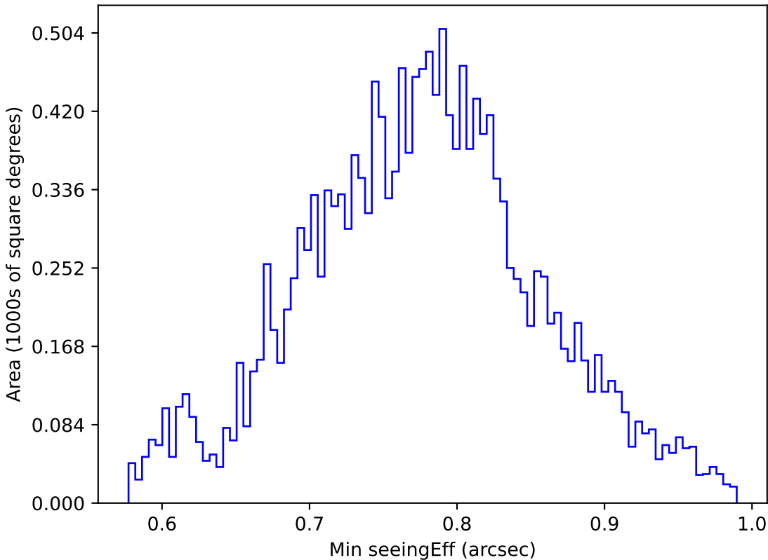
roll_pause_mjdp60_v3.4_10yrs WFD u band: Min seeingEff
