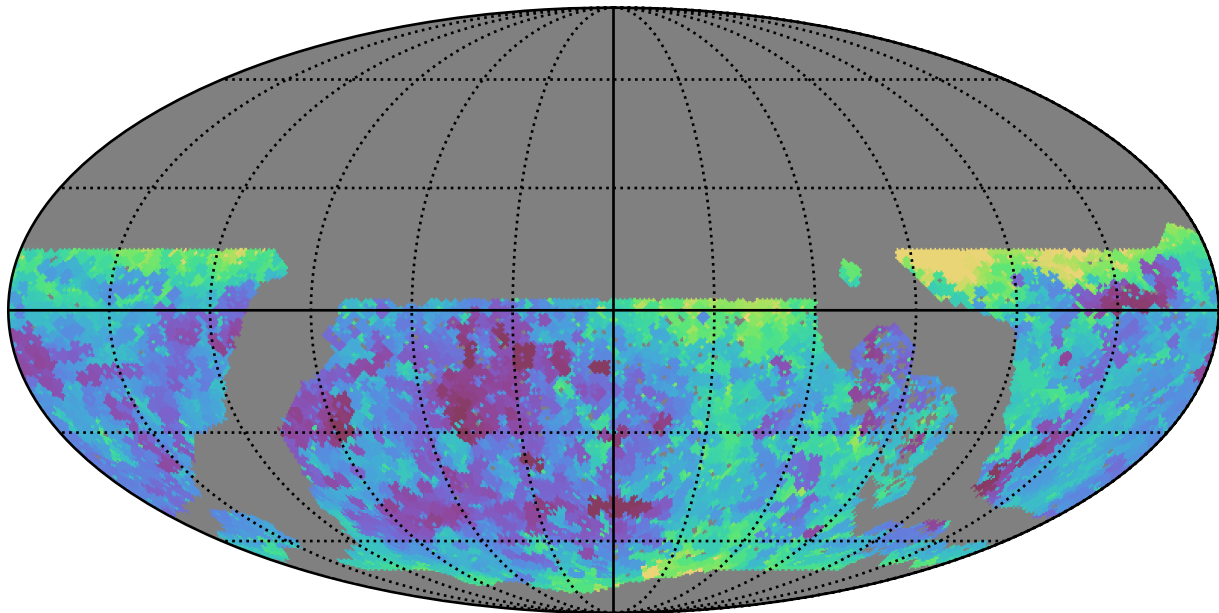
roll_pause_mjdp60_v3.4_10yrs WFD r band: Min seeingEff
