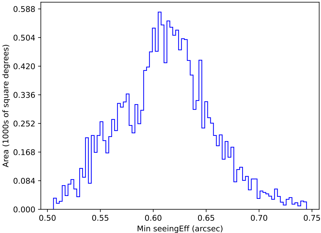
roll_pause_mjdp60_v3.4_10yrs WFD r band: Min seeingEff
