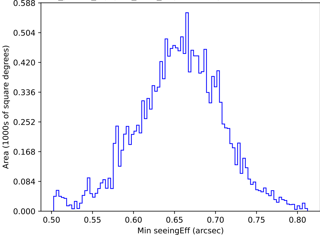
roll_pause_mjdp60_v3.4_10yrs WFD g band: Min seeingEff
