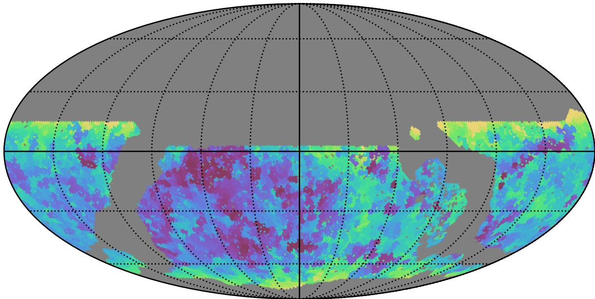
roll_pause_mjdp60_v3.4_10yrs WFD all bands: Min seeingEff
