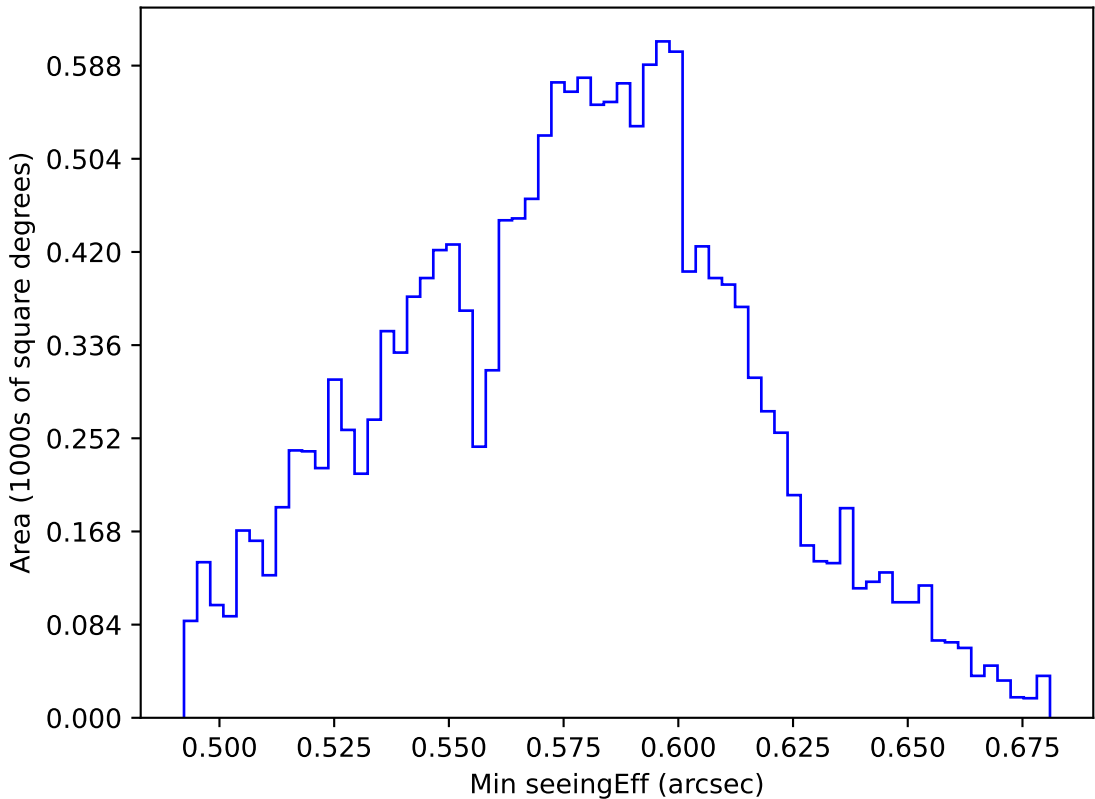
roll_pause_mjdp60_v3.4_10yrs WFD all bands: Min seeingEff
