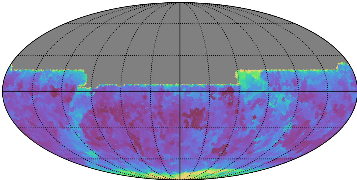
roll_pause_mjdp60_v3.4_10yrs All sky y band: Min seeingEff
