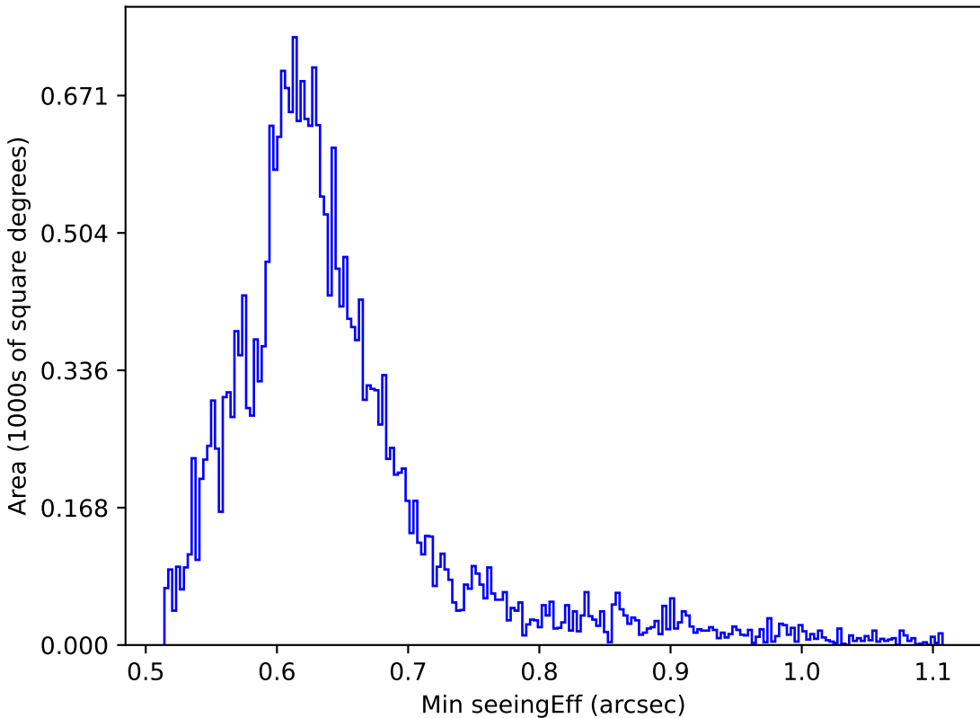
roll_pause_mjdp60_v3.4_10yrs All sky r band: Min seeingEff
