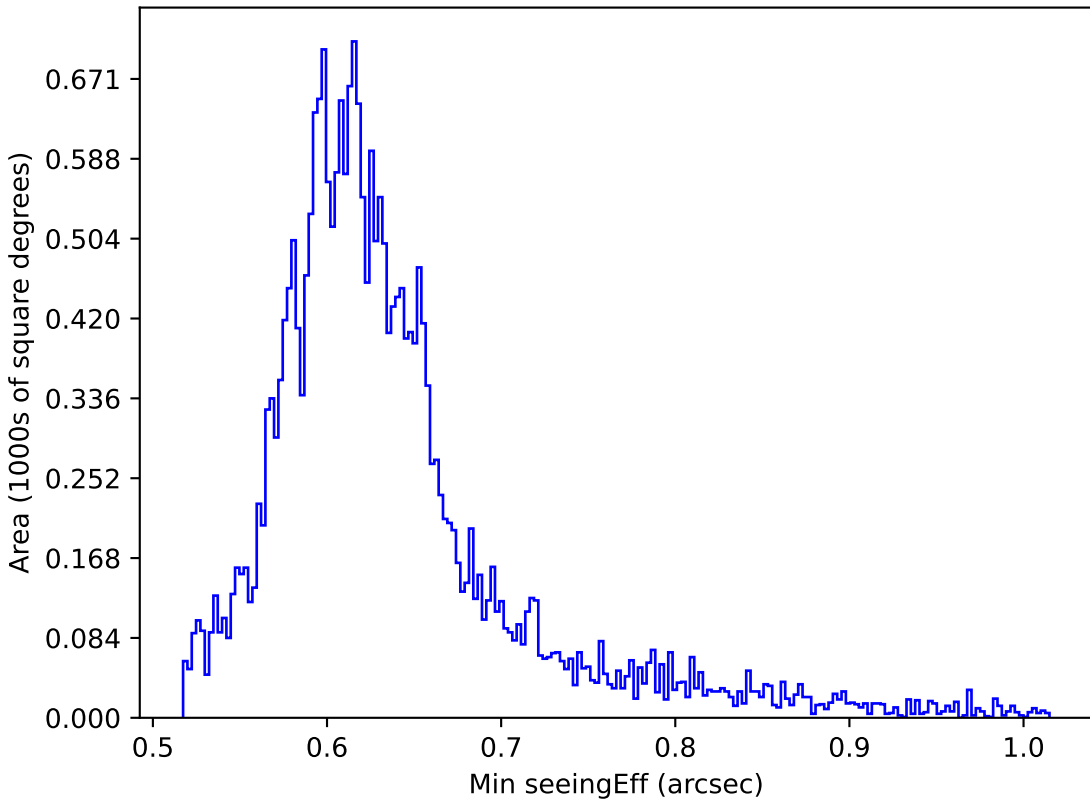
roll_pause_mjdp60_v3.4_10yrs All sky i band: Min seeingEff
