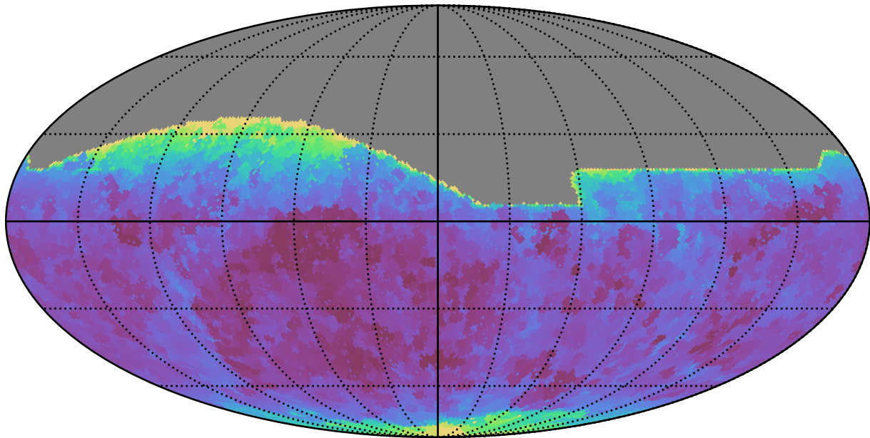
roll_pause_mjdp60_v3.4_10yrs All sky all bands: Min seeingEff
