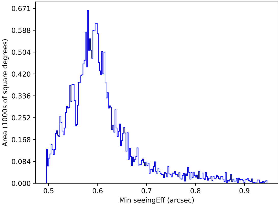
roll_pause_mjdp60_v3.4_10yrs All sky all bands: Min seeingEff
