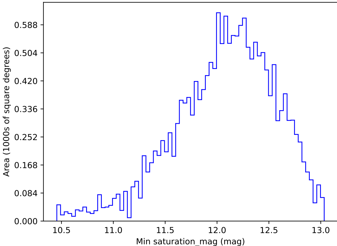
roll_pause_mjdp60_v3.4_10yrs WFD z band: Min saturation_mag
