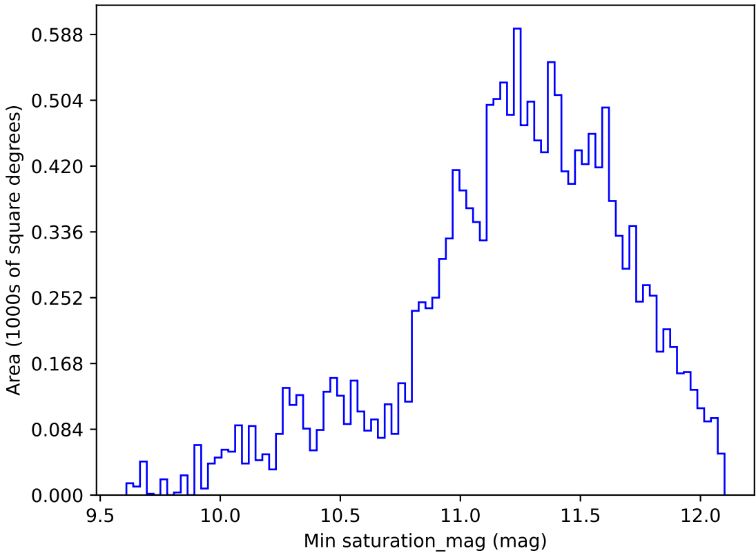
roll_pause_mjdp60_v3.4_10yrs WFD y band: Min saturation_mag
