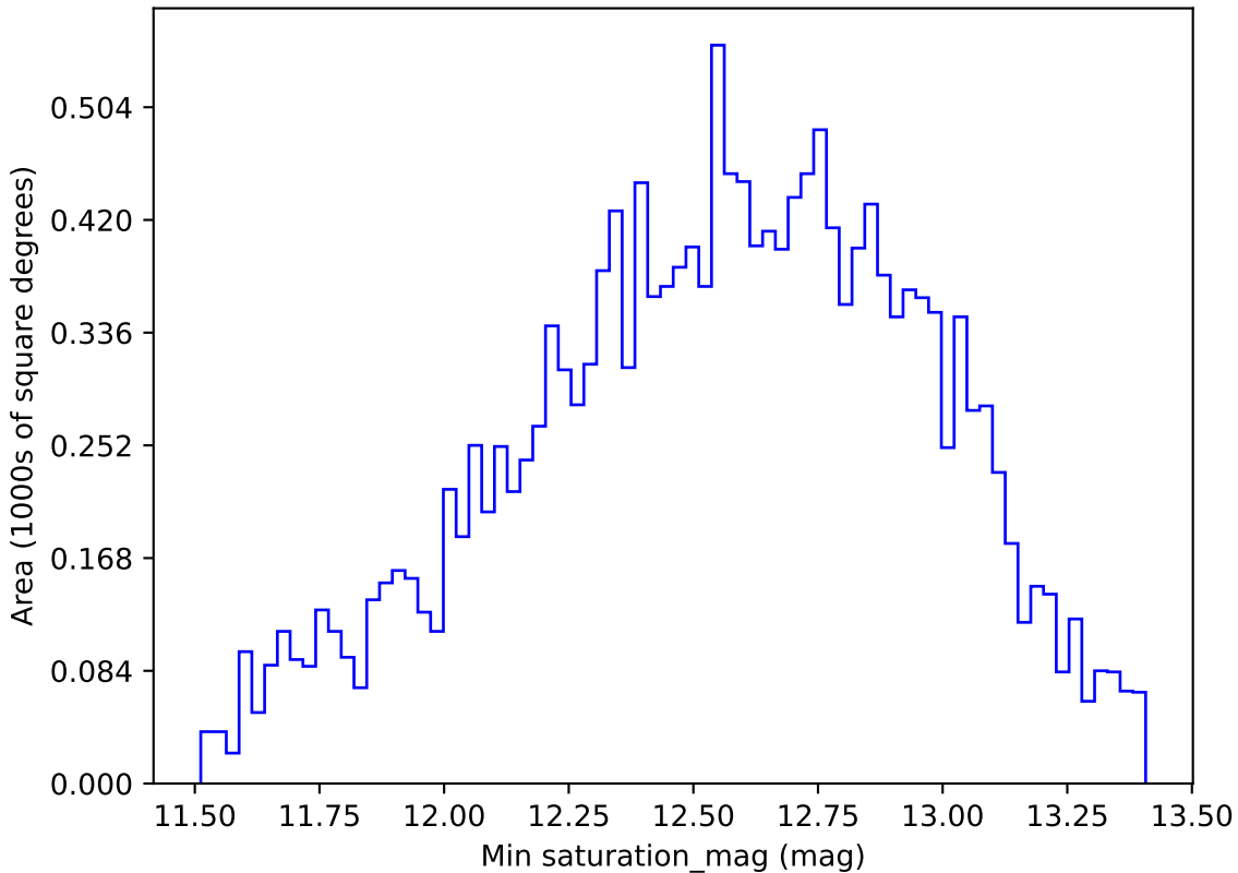
roll_pause_mjdp60_v3.4_10yrs WFD r band: Min saturation_mag
