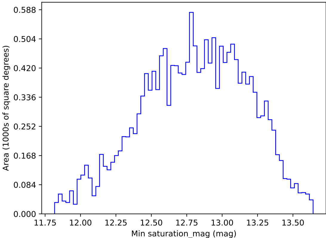
roll_pause_mjdp60_v3.4_10yrs WFD g band: Min saturation_mag
