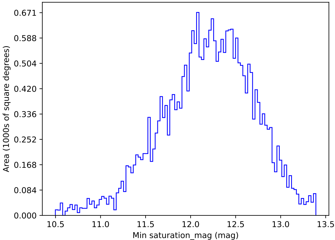
roll_pause_mjdp60_v3.4_10yrs All sky z band: Min saturation_mag
