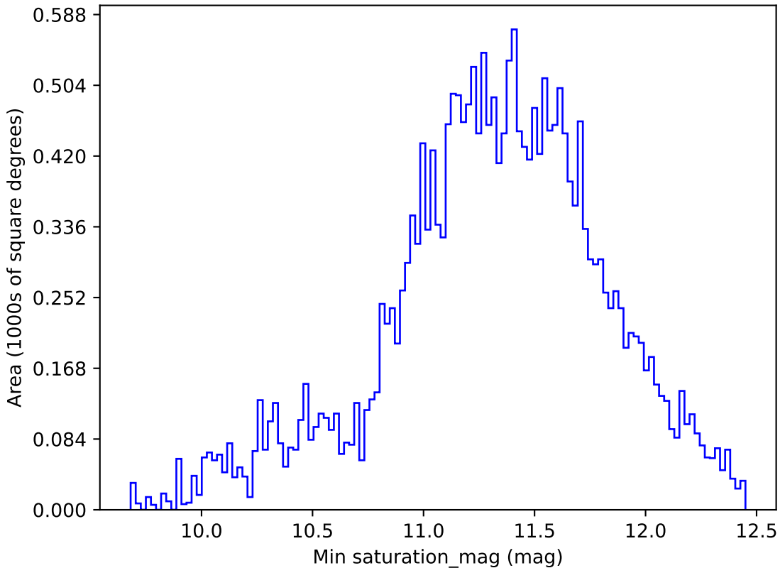
roll_pause_mjdp60_v3.4_10yrs All sky y band: Min saturation_mag
