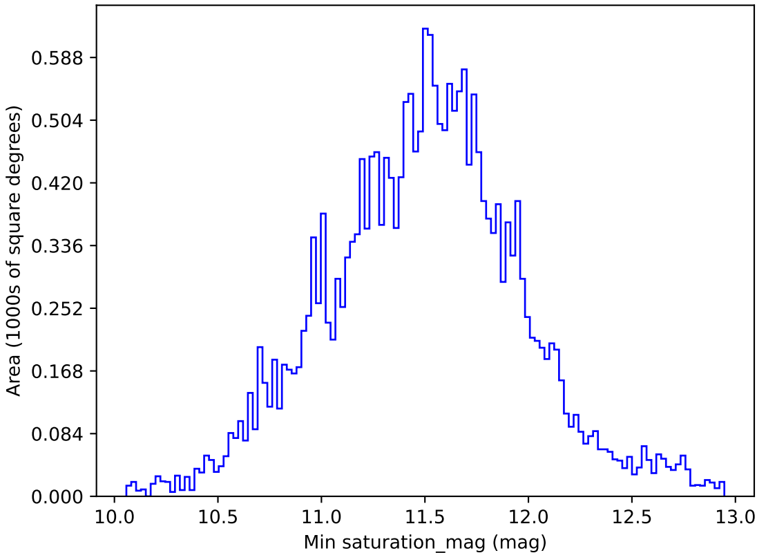
roll_pause_mjdp60_v3.4_10yrs All sky u band: Min saturation_mag
