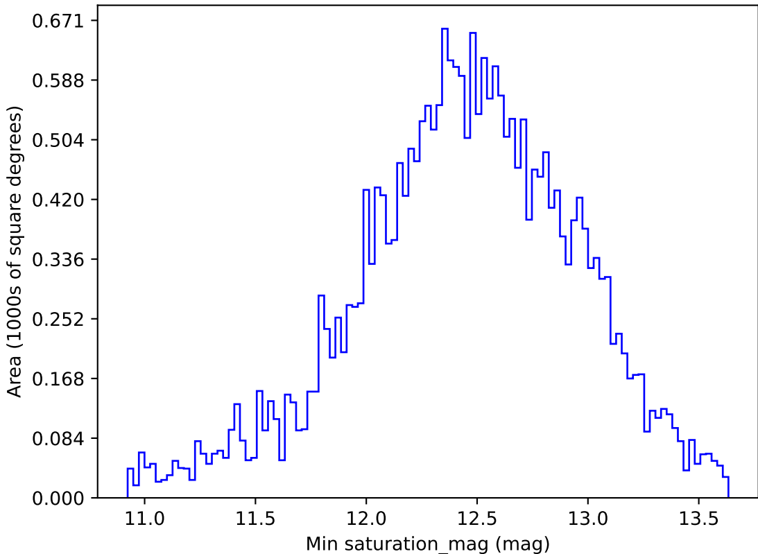
roll_pause_mjdp60_v3.4_10yrs All sky i band: Min saturation_mag
