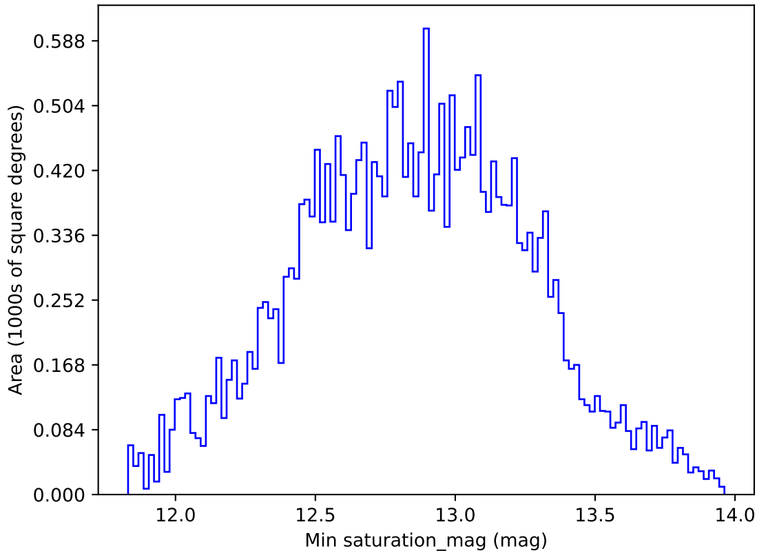
roll_pause_mjdp60_v3.4_10yrs All sky g band: Min saturation_mag
