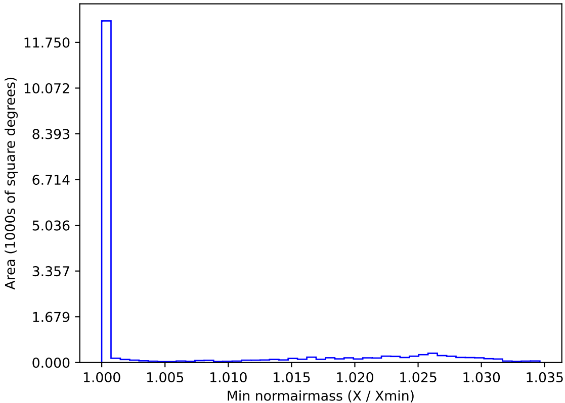
roll_pause_mjdp60_v3.4_10yrs WFD z band: Min normairmass
