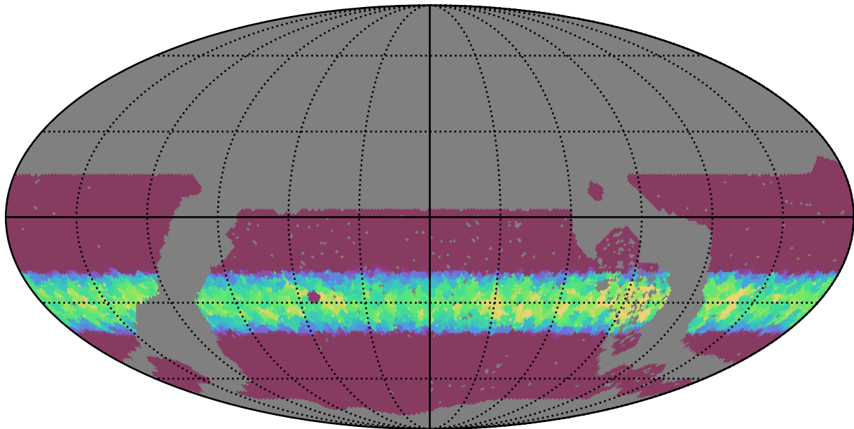
roll_pause_mjdp60_v3.4_10yrs WFD y band: Min normairmass
