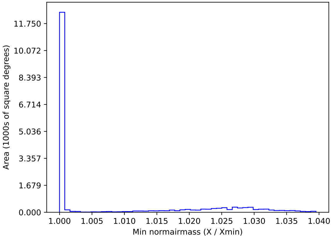
roll_pause_mjdp60_v3.4_10yrs WFD y band: Min normairmass
