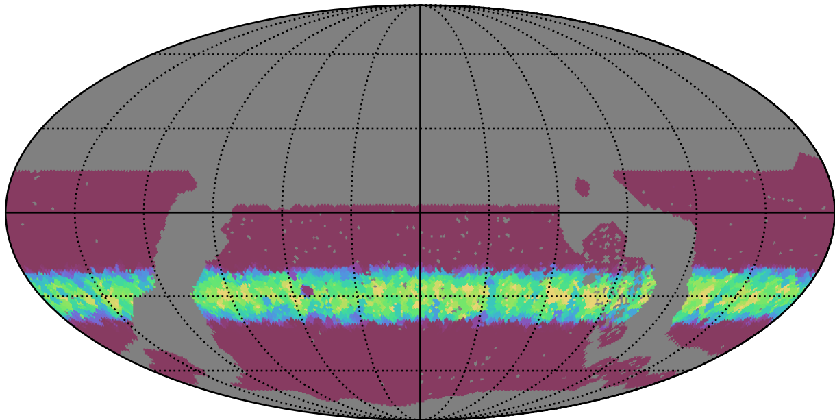
roll_pause_mjdp60_v3.4_10yrs WFD r band: Min normairmass
