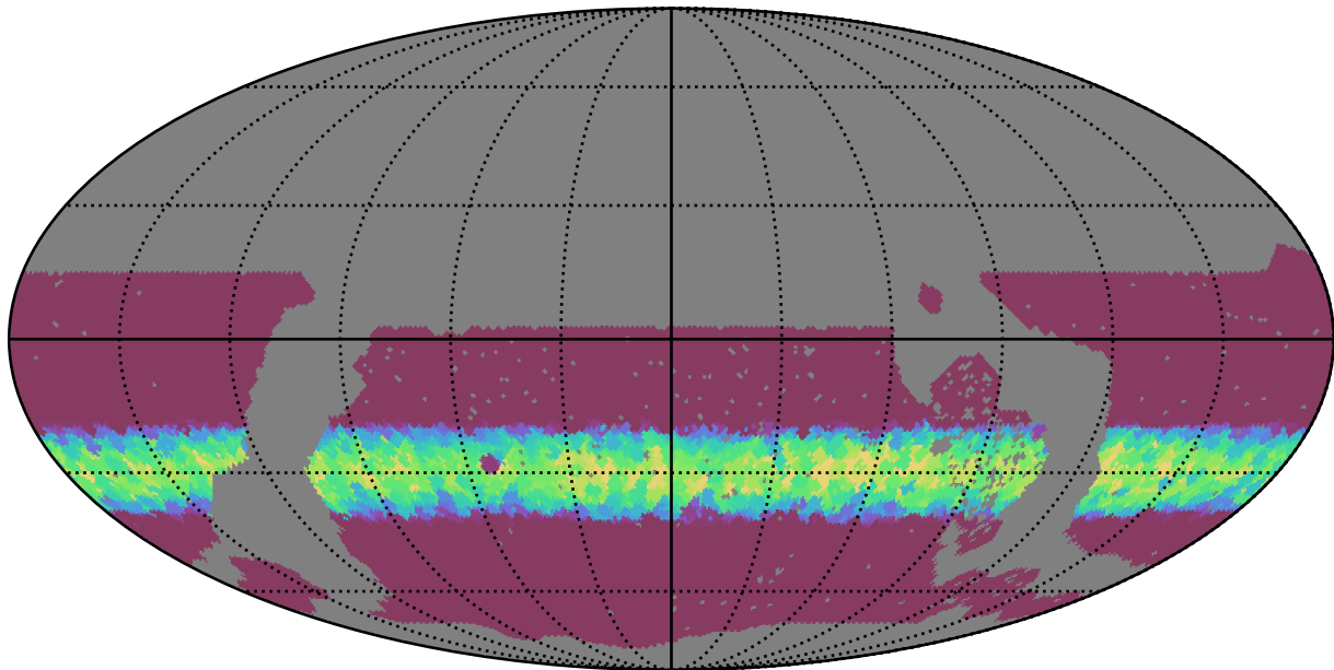
roll_pause_mjdp60_v3.4_10yrs WFD i band: Min normairmass
